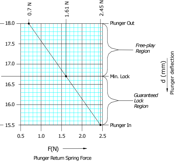
AL1 Nominal Internal spring characteristic *Excluding Tolerance and friction
